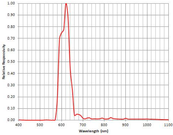
SPECTRAL RESPONSE (Ta=23°C)
