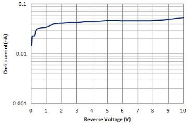
DARK CURRENT VS. REVERSE VOLTAGE(Ta=23°C)
