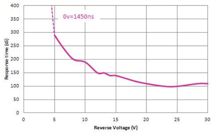
RISE TIME *VS. REVERSE VOLTAGE (Ta=23°C)
