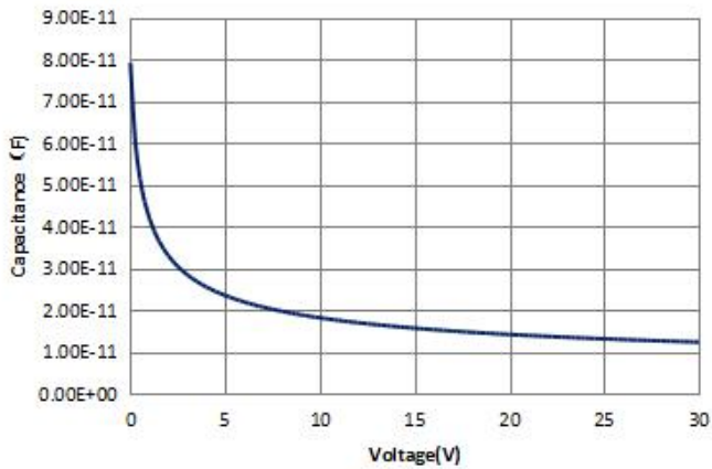
CAPACITANCE VS. REVERSE VOLTAGE (Ta=23°C)
