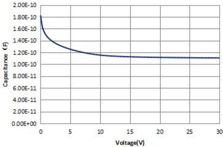
CAPACITANCE VS. REVERSE VOLTAGE (Ta=23°C)
