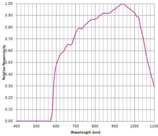
SPECTRAL RESPONSE (Ta=23°C)
