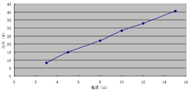
Forward current Vs. Peak power(Ta=25°C)
