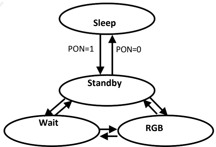
< State machine >
